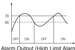
Alarm Output (High Limit Alarm) [AtS=70, AdF=5, AdL=0, SAo=0]
