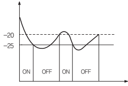
Main output [setting=-25 °C, dlf=5, dLy=0, tyP=CoL]
