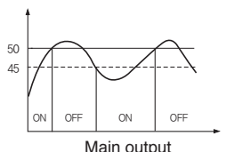
Main output [setting=50 °C, dlf=5, dLy=0, tyP=HEt]
