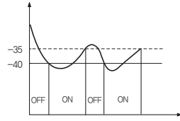
Alarm Output (Low Limit Alarm) [AtS=-40, AdF=5, AdL=0, SAo=0]
